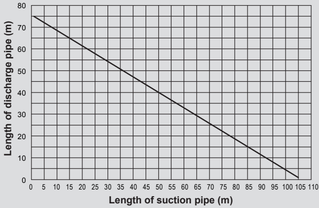
Maximum pipe length Ø 80 mm - 25 KIS
