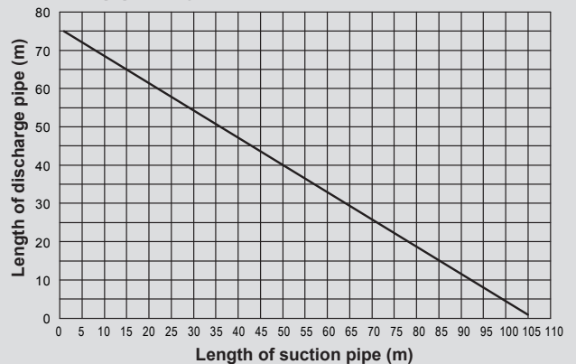
Maximum pipe length Ø 80 mm - 25 KIS
