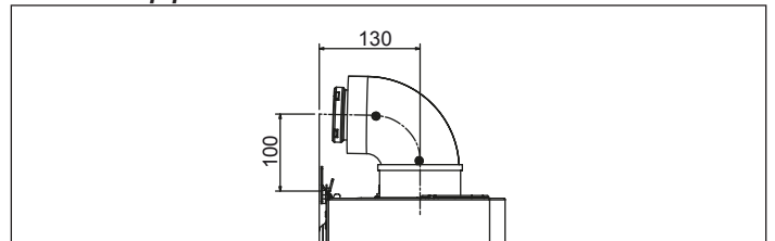
Twin pipes ø 80mm
