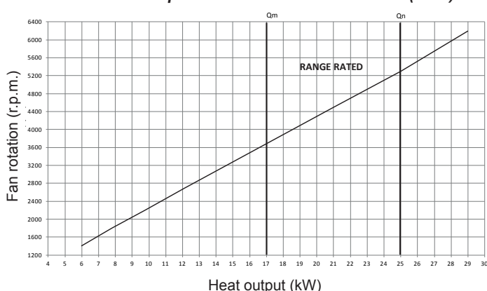
Thermal output curve - no. of fan rotations (MTN)
