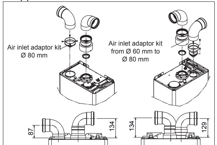
Twin pipes ø 80mm
