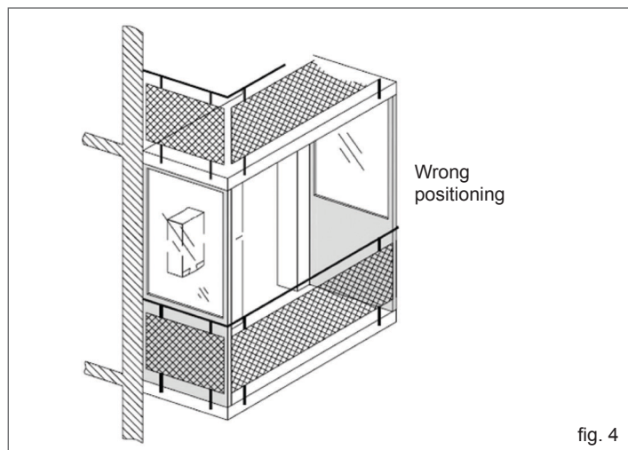
Fig. 4: example of INCORRECT expulsion of combustion products inside a balcony closed on five sides.
